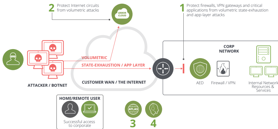
Figure 2: Arbor Smart DDoS Protection Enables Remote/Home User Access to Corporate Resources.
